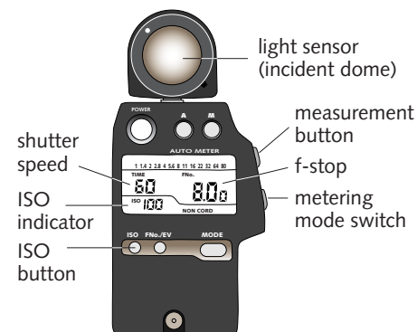
Digital incident-light meter
