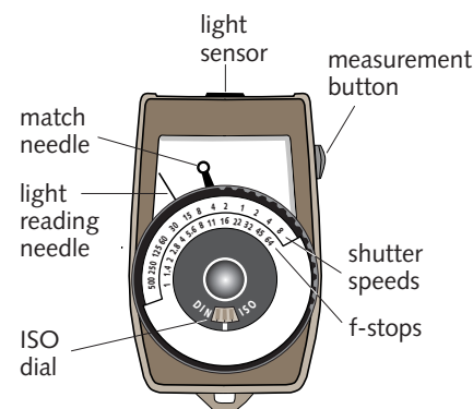
Analog reflected-light meter
