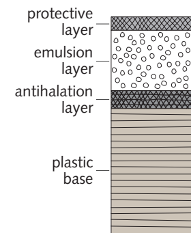
Cross section of black-and-white film
